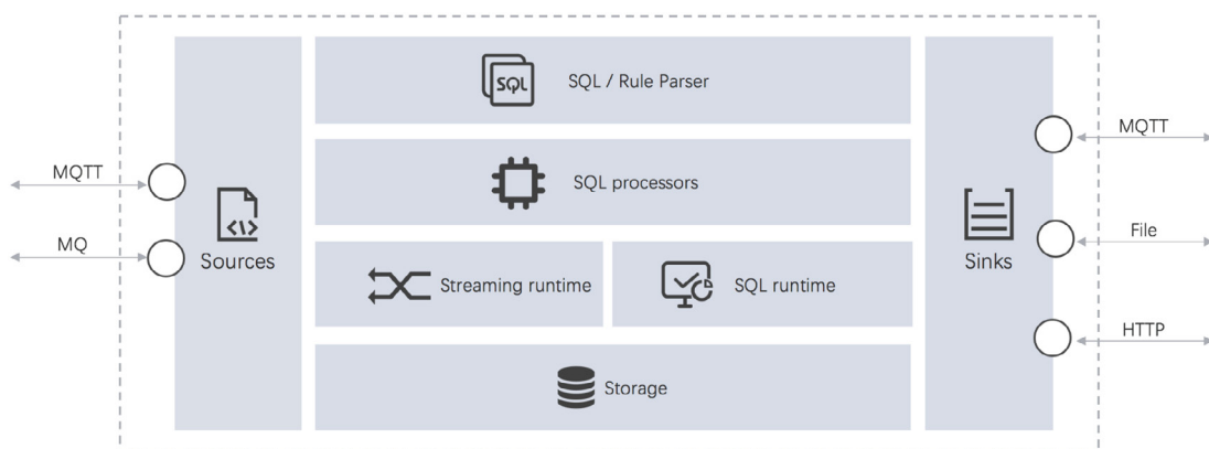
eKuiper Architecture
