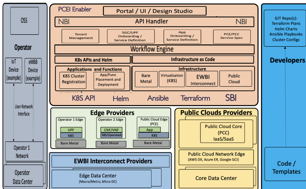
Akraïno PCEI Blueprint Architecture
