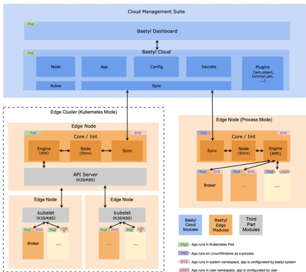
Baetyl Architecture
