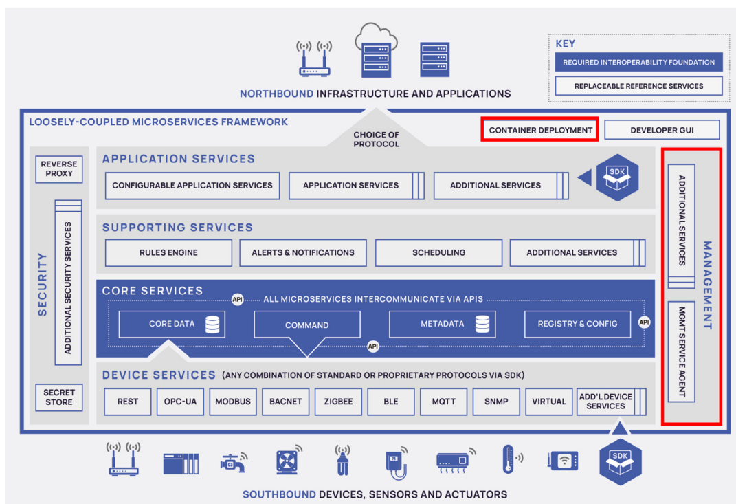
EdgeX Foundry System Management Services
