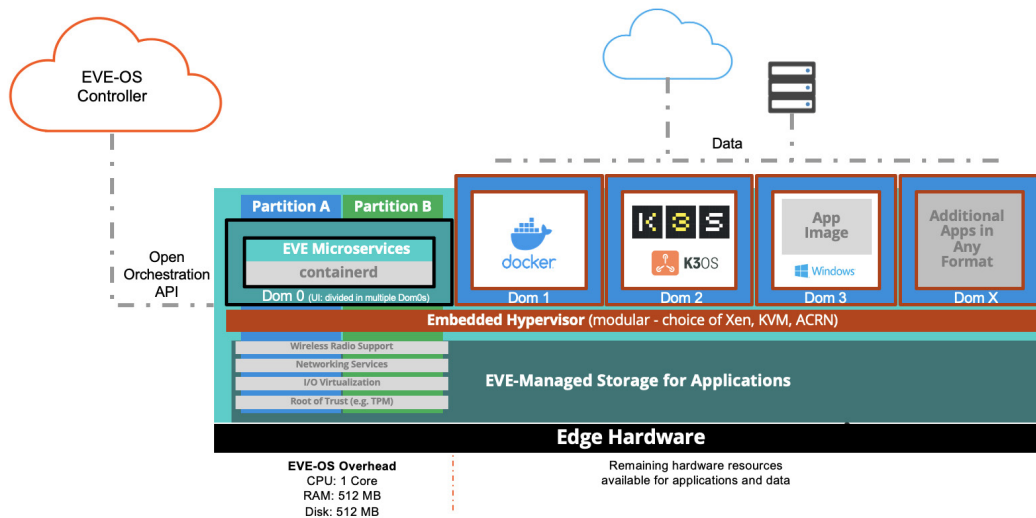
EVE-OS Architecture
