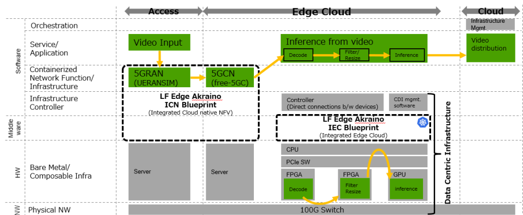
FIGURE 7: IOWN GF/LF EDGE JOINT POC DETAILS
