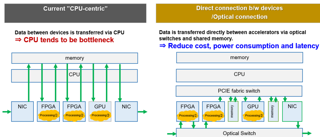
FIGURE 5: DIRECT TRANSFER BETWEEN ACCELERATOR DEVICES
